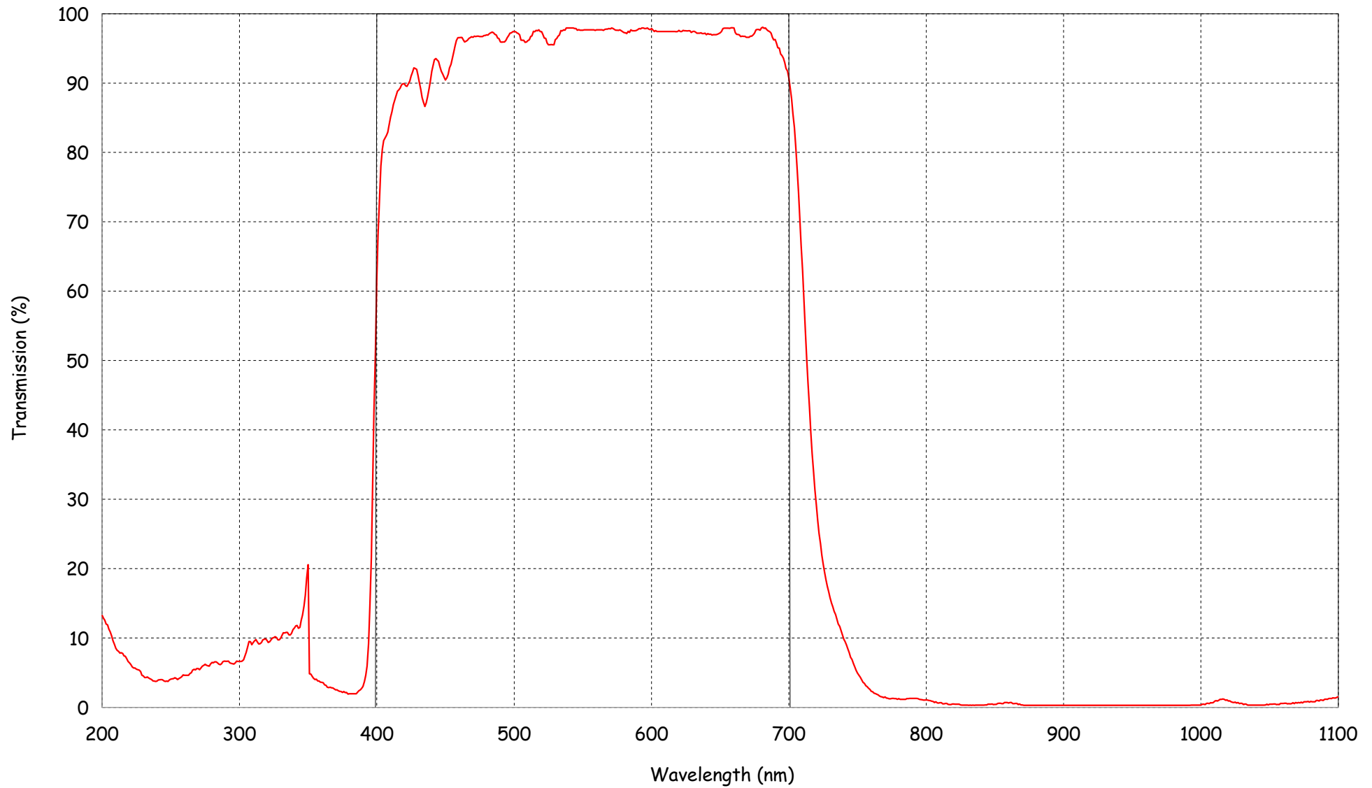
FHBB - F Hot mirror 720nm + AR 1 Lato - boroglass 1mm thck
